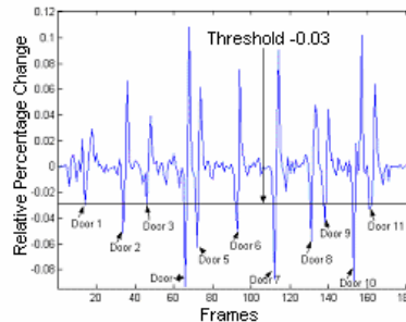
Figure 17: Plot showing the doors recognized.
